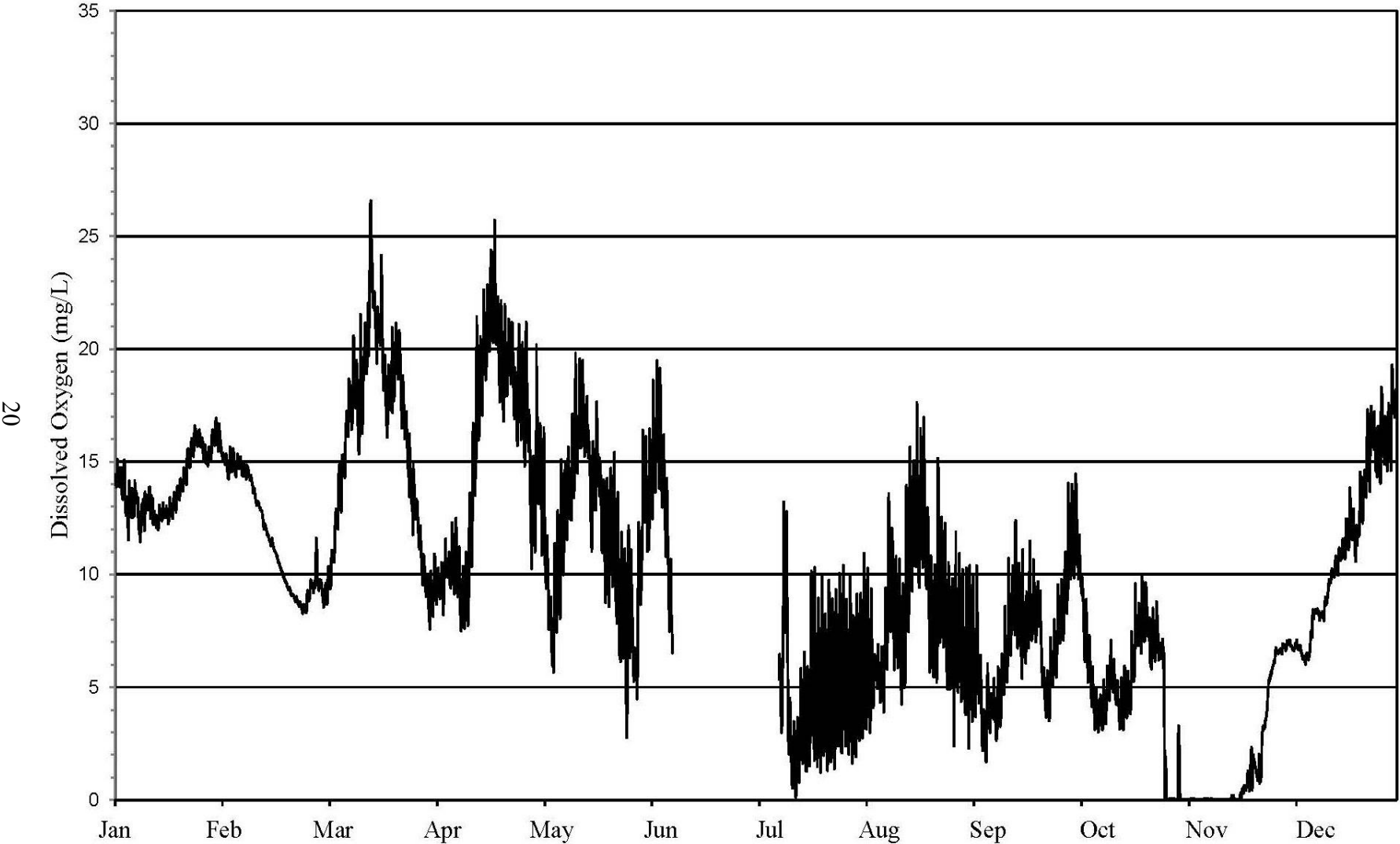
FIGURE 8: DISSOLVED OXYGEN CONCENTRATION MEASURED HOURLY AT 36TH STREET ON BUBBLY CREEK FROM JANUARY 1, 2021 THROUGH DECEMBER 31, 2021
