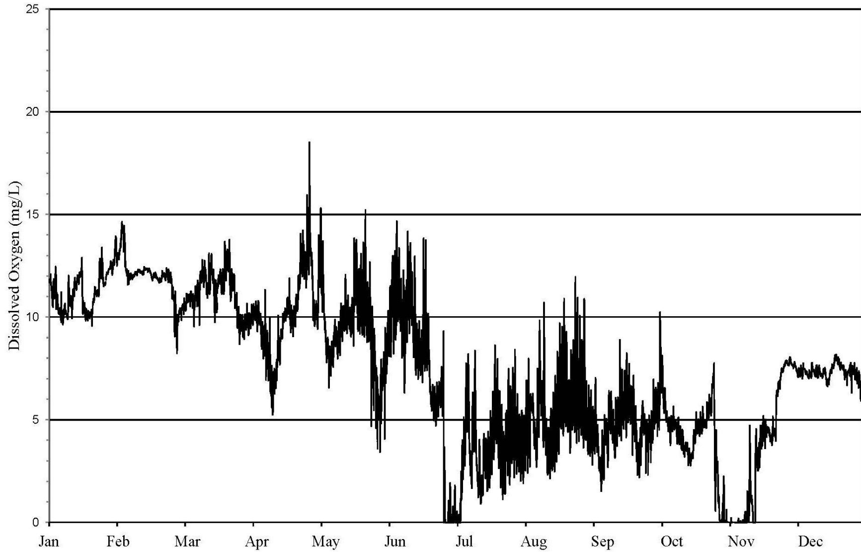
FIGURE 9: DISSOLVED OXYGEN CONCENTRATION MEASURED HOURLY AT INTERSTATE HIGHWAY 55 ON BUBBLY CREEK FROM JANUARY 1, 2021 THROUGH DECEMBER 31, 2021
