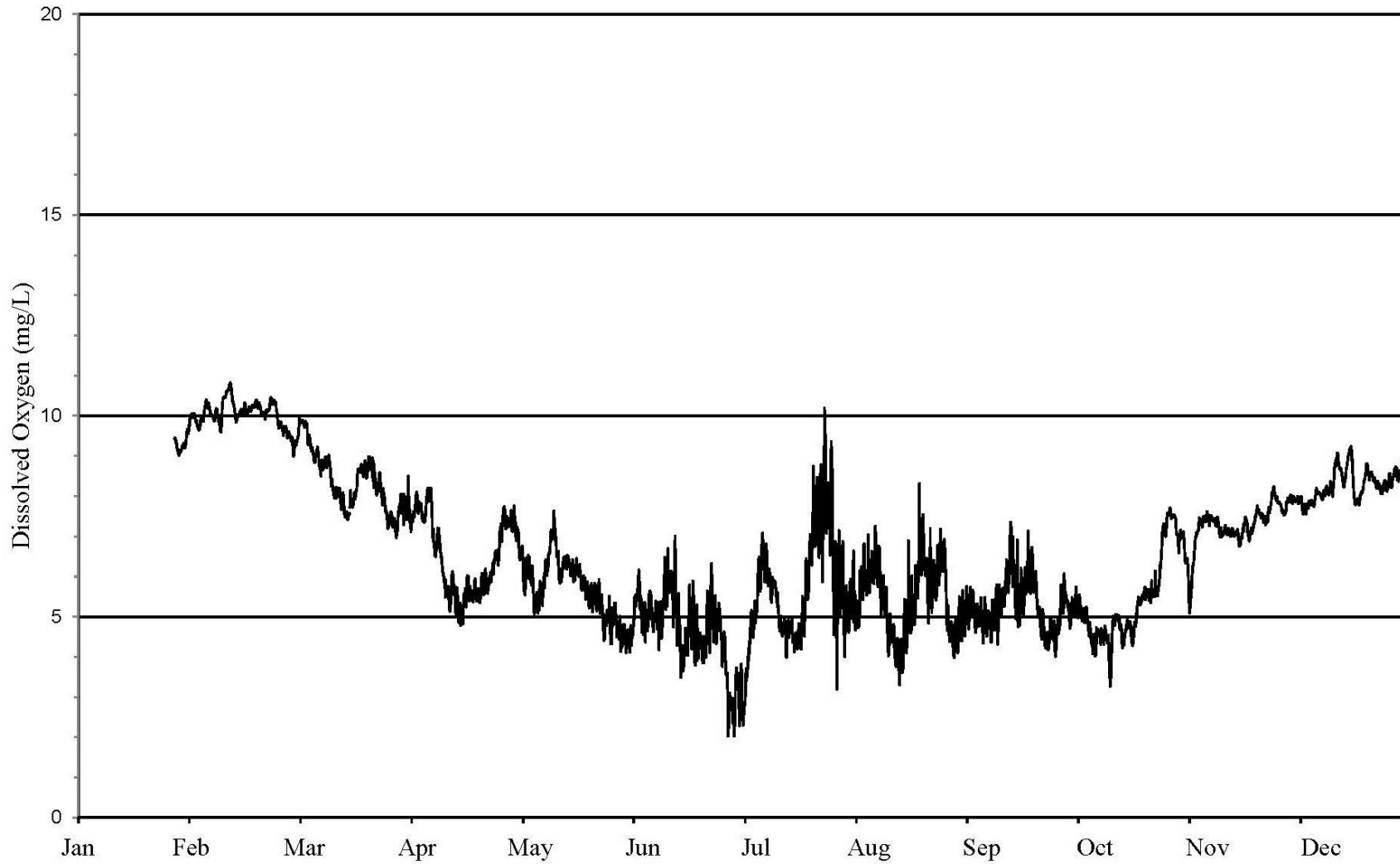
FIGURE 12: DISSOLVED OXYGEN CONCENTRATION MEASURED HOURLY AT LOCKPORT POWERHOUSE ON THE CHICAGO SANITARY AND SHIP CANAL FROM JANUARY 1, 2021 THROUGH DECEMBER 31, 2021
