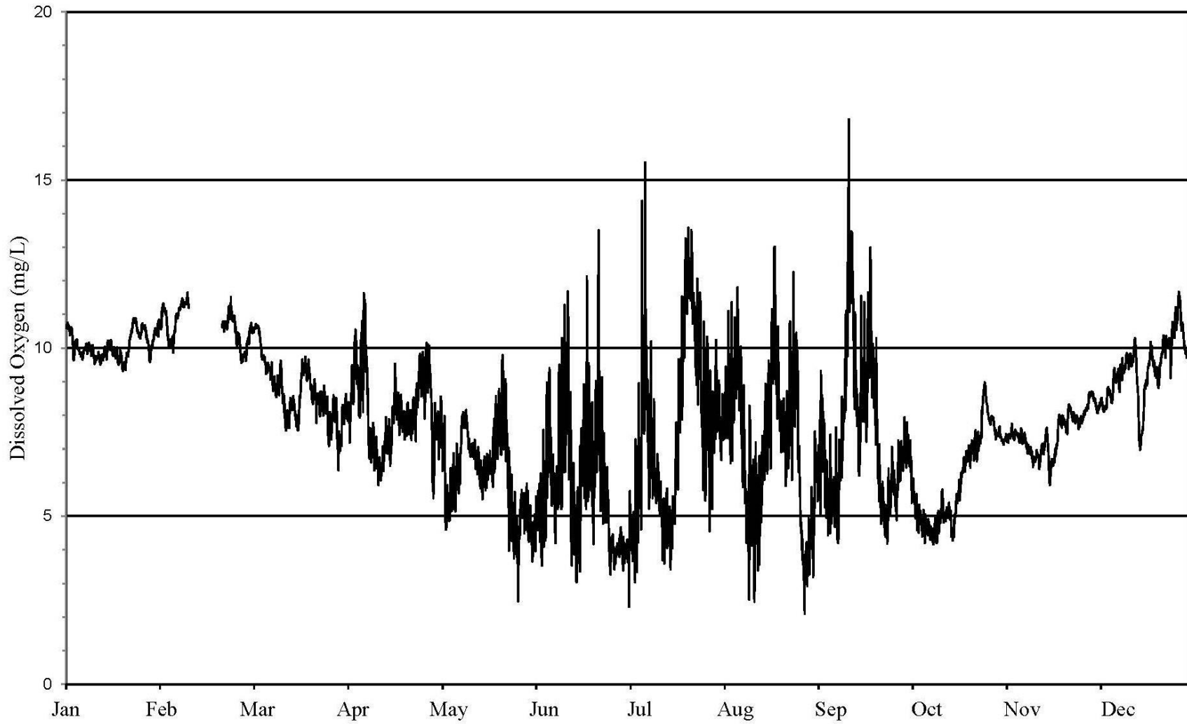
FIGURE 17: DISSOLVED OXYGEN CONCENTRATION MEASURED HOURLY AT ROUTE 83 ON THE CALUMET-SAG CHANNEL FROM JANUARY 1, 2021 THROUGH DECEMBER 31, 2021
