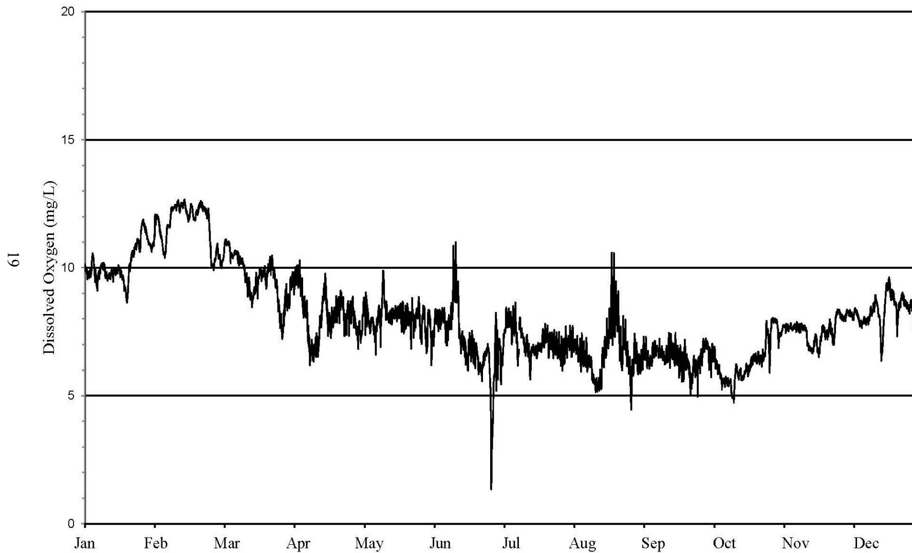
FIGURE 7: DISSOLVED OXYGEN CONCENTRATION MEASURED HOURLY AT LOOMIS STREET ON THE SOUTH BRANCH OF THE CHICAGO RIVER FROM JANUARY 1, 2021 THROUGH DECEMBER 31, 2021
