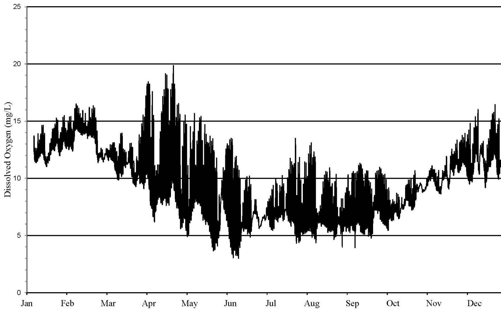
FIGURE 21: DISSOLVED OXYGEN CONCENTRATION MEASURED HOURLY AT WOLF ROAD ON SALT CREEK FROM JANUARY 1, 2021 THROUGH DECEMBER 31, 2021
