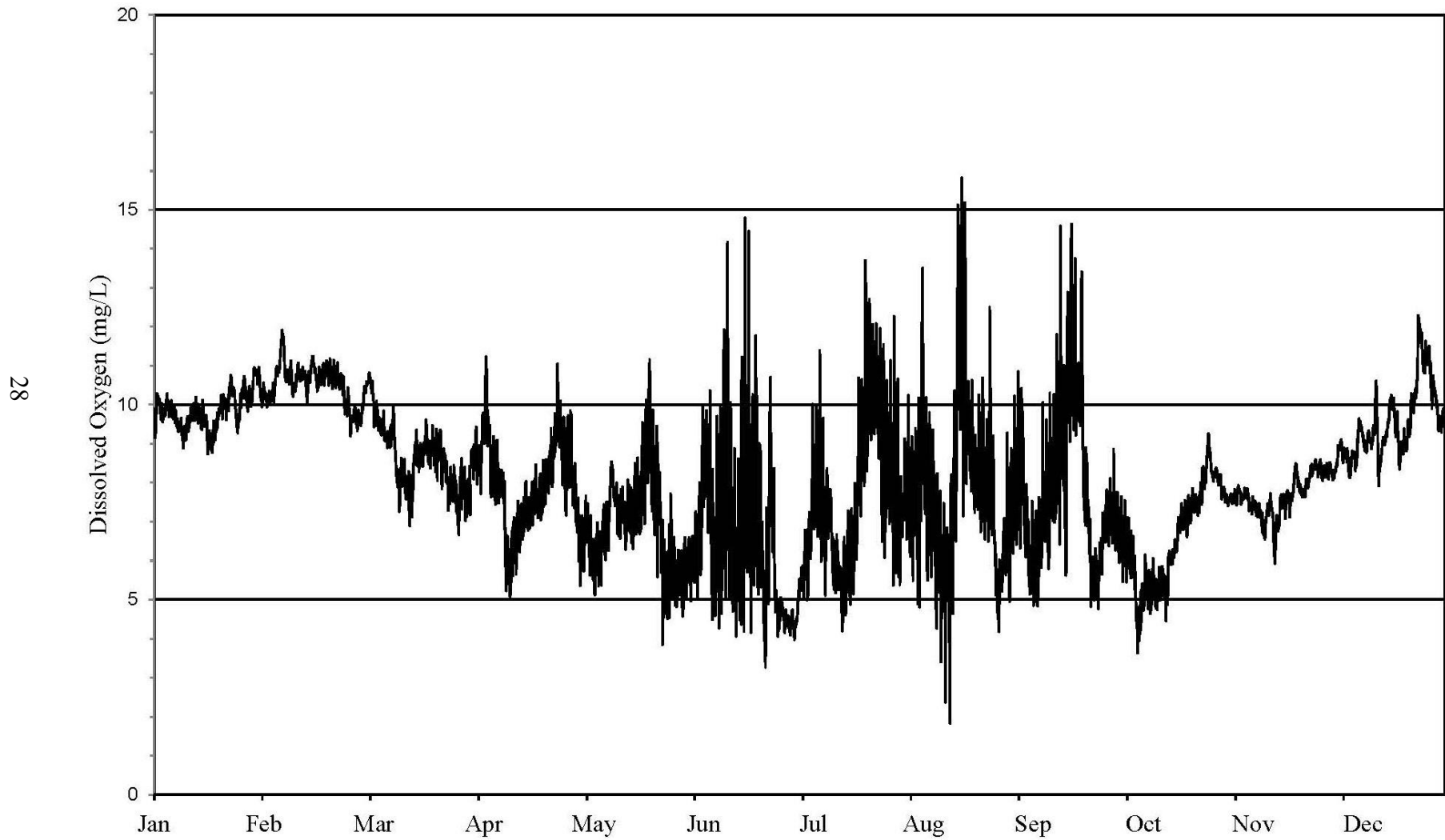
FIGURE 16: DISSOLVED OXYGEN CONCENTRATION MEASURED HOURLY AT CICERO AVENUE ON THE CALUMET-SAG CHANNEL FROM JANUARY 1, 2021 THROUGH DECEMBER 31, 2021
