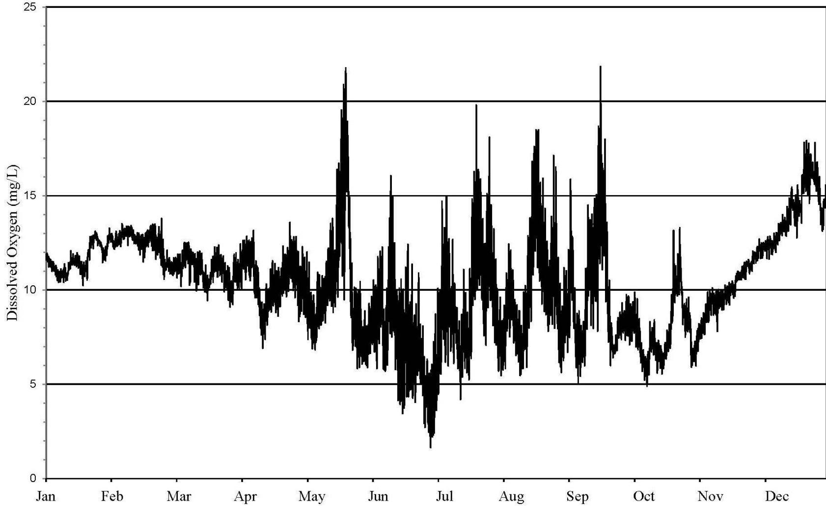
FIGURE 13: DISSOLVED OXYGEN CONCENTRATION MEASURED HOURLY AT C&W INDIANA RAILROAD ON THE LITTLE CALUMET RIVER FROM JANUARY 1, 2021 THROUGH DECEMBER 31, 2021
