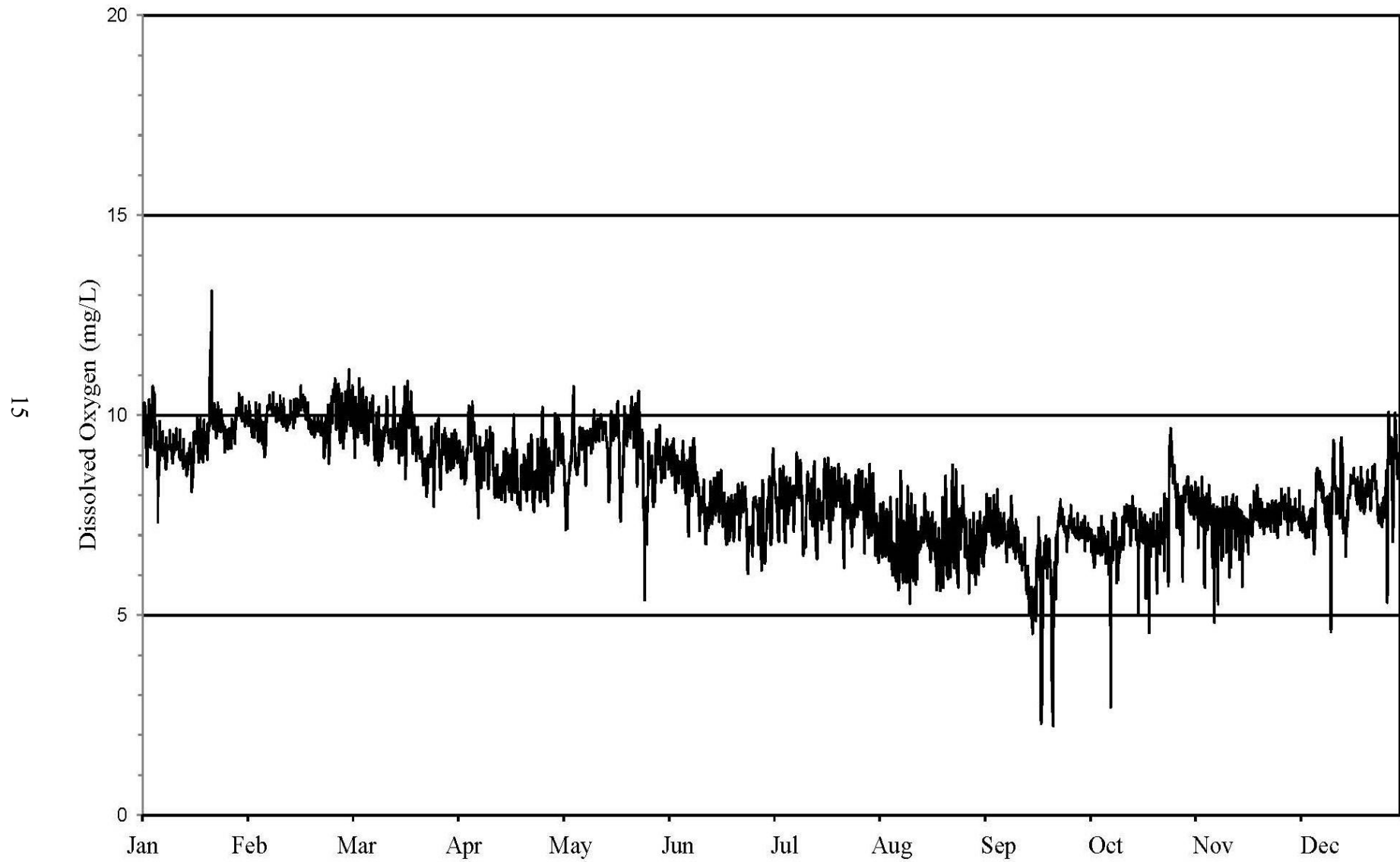
FIGURE 3: DISSOLVED OXYGEN CONCENTRATION MEASURED HOURLY AT FOSTER AVENUE ON THE NORTH SHORE CHANNEL FROM JANUARY 1, 2021 THROUGH DECEMBER 31, 2021
