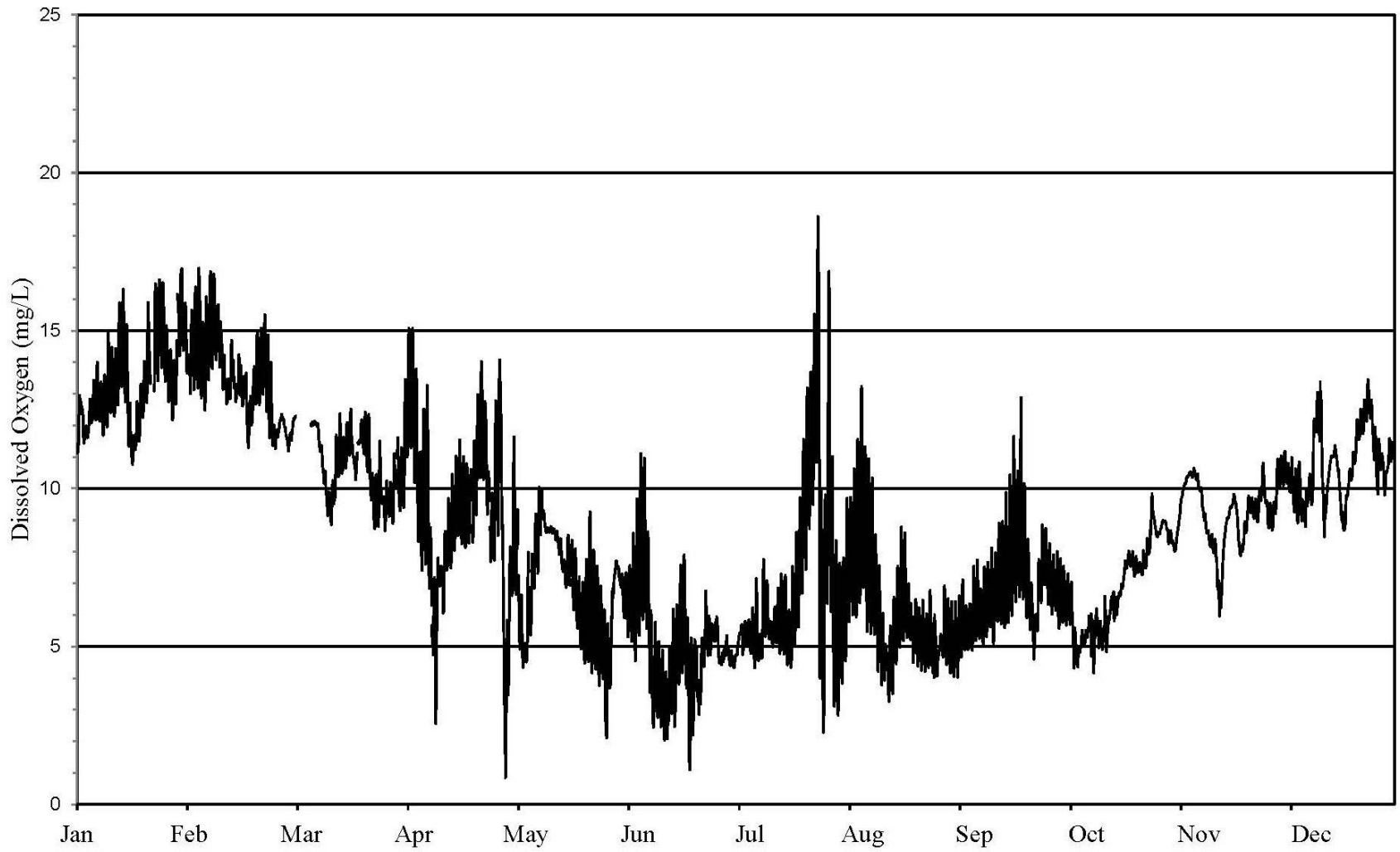
FIGURE 15: DISSOLVED OXYGEN CONCENTRATION MEASURED HOURLY AT ASHLAND AVENUE ON THE LITTLE CALUMET RIVER FROM JANUARY 1, 2021 THROUGH DECEMBER 31, 2021
