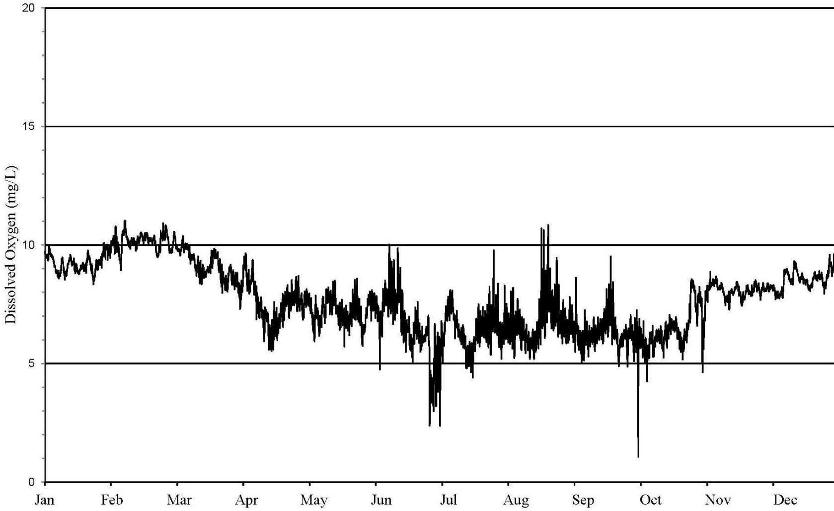
FIGURE 11: DISSOLVED OXYGEN CONCENTRATION MEASURED HOURLY AT B&O RAILROAD ON THE SANITARY AND SHIP CANAL FROM JANUARY 1, 2021 THROUGH DECEMBER 31, 2021
