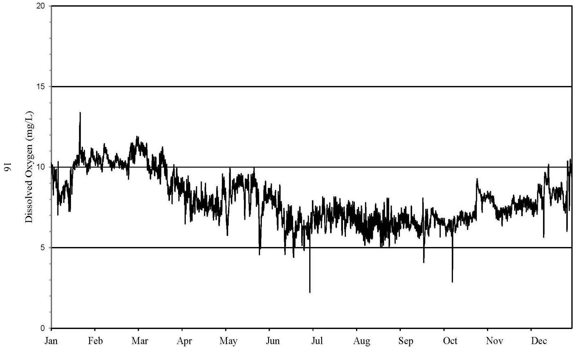
FIGURE 4: DISSOLVED OXYGEN CONCENTRATION MEASURED HOURLY AT ADDISON STREET ON THE NORTH BRANCH CHICAGO RIVER FROM JANUARY 1, 2021 THROUGH DECEMBER 31, 2021
