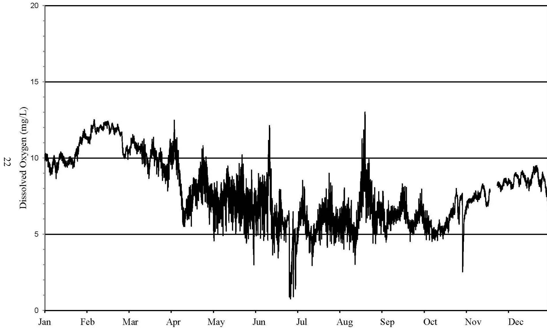
FIGURE 10: DISSOLVED OXYGEN CONCENTRATION MEASURED HOURLY AT CICERO AVENUE ON THE CHICAGO SANITARY AND SHIP CANAL FROM JANUARY 1, 2021 THROUGH DECEMBER 31, 2021
