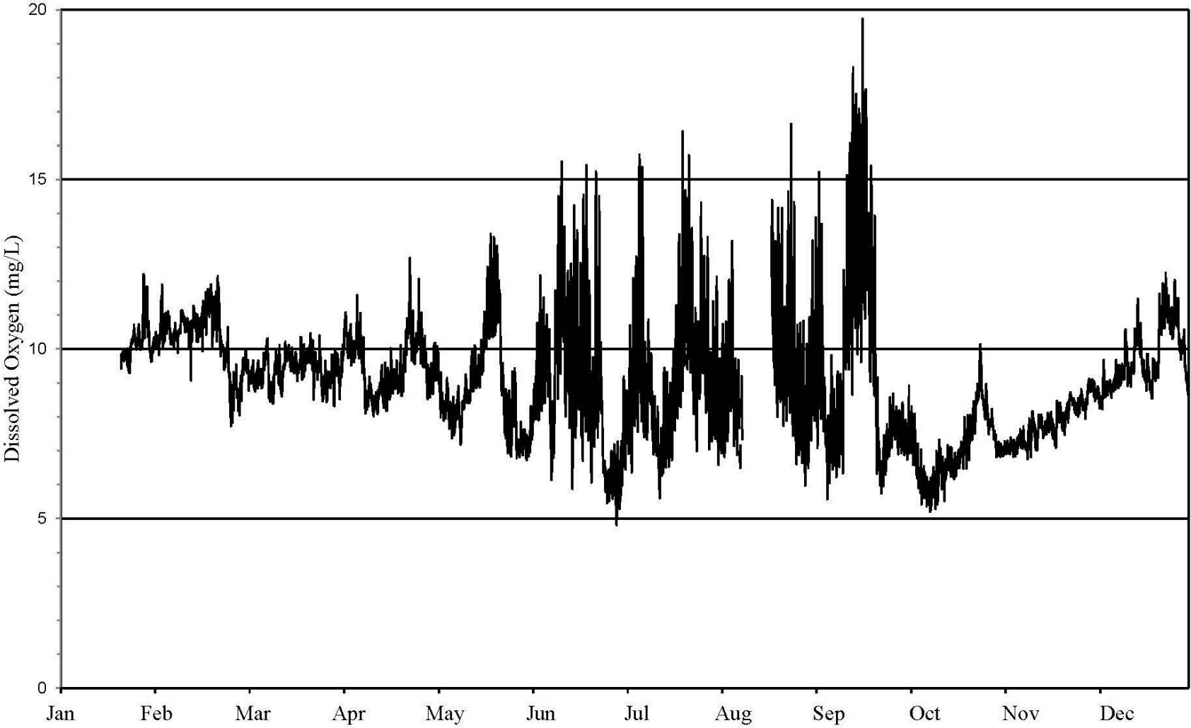
FIGURE 14: DISSOLVED OXYGEN CONCENTRATION MEASURED HOURLY AT HALSTED STREET ON THE LITTLE CALUMET RIVER FROM JANUARY 1, 2021 THROUGH DECEMBER 31, 2021
