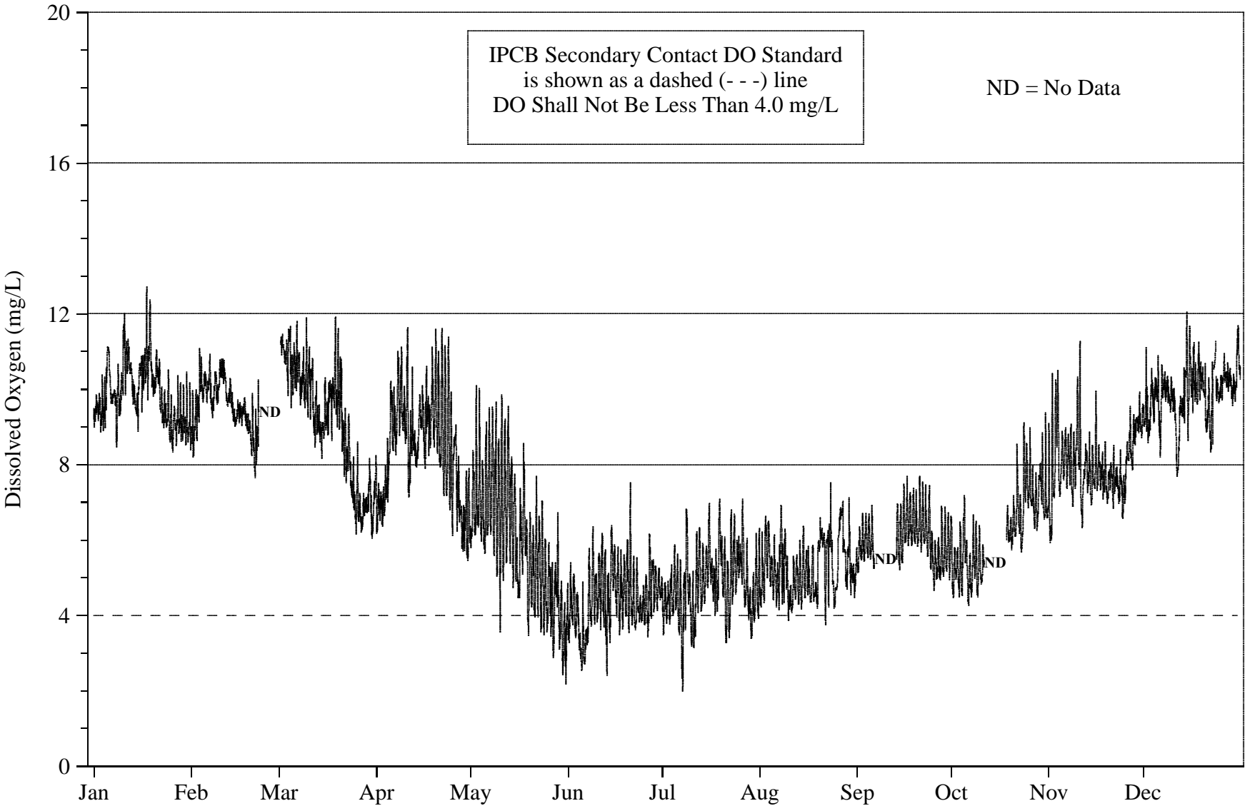
FIGURE 15: DISSOLVED OXYGEN CONCENTRATION MEASURED HOURLY AT JEFFERSON STREET ON THE DES PLAINES RIVER FROM JANUARY 2007 THROUGH DECEMBER 2007
