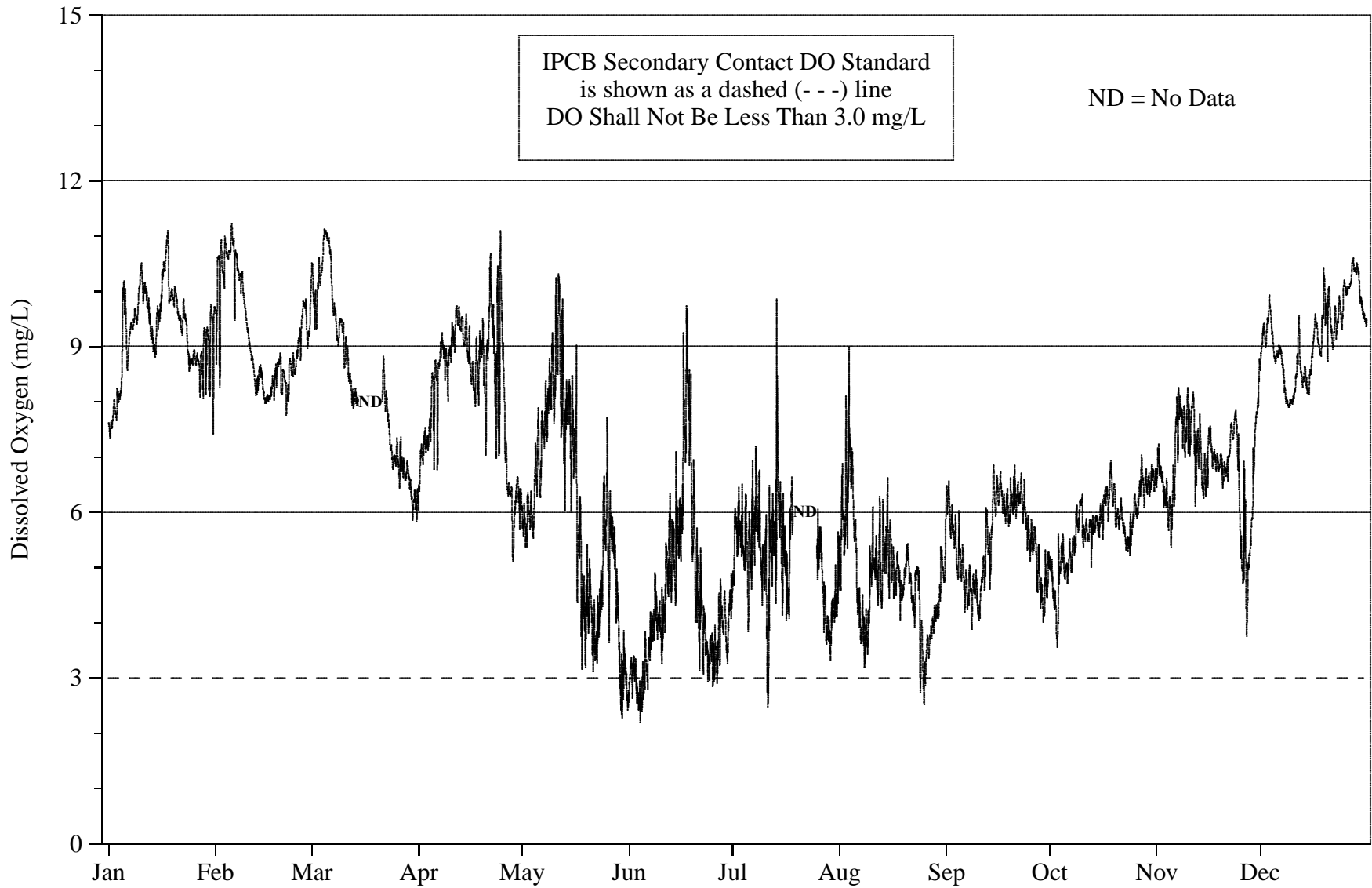
FIGURE 20: DISSOLVED OXYGEN CONCENTRATION MEASURED HOURLY AT ROUTE 83 ON THE CALUMET-SAG CHANNEL FROM JANUARY 2007 THROUGH DECEMBER 2007
