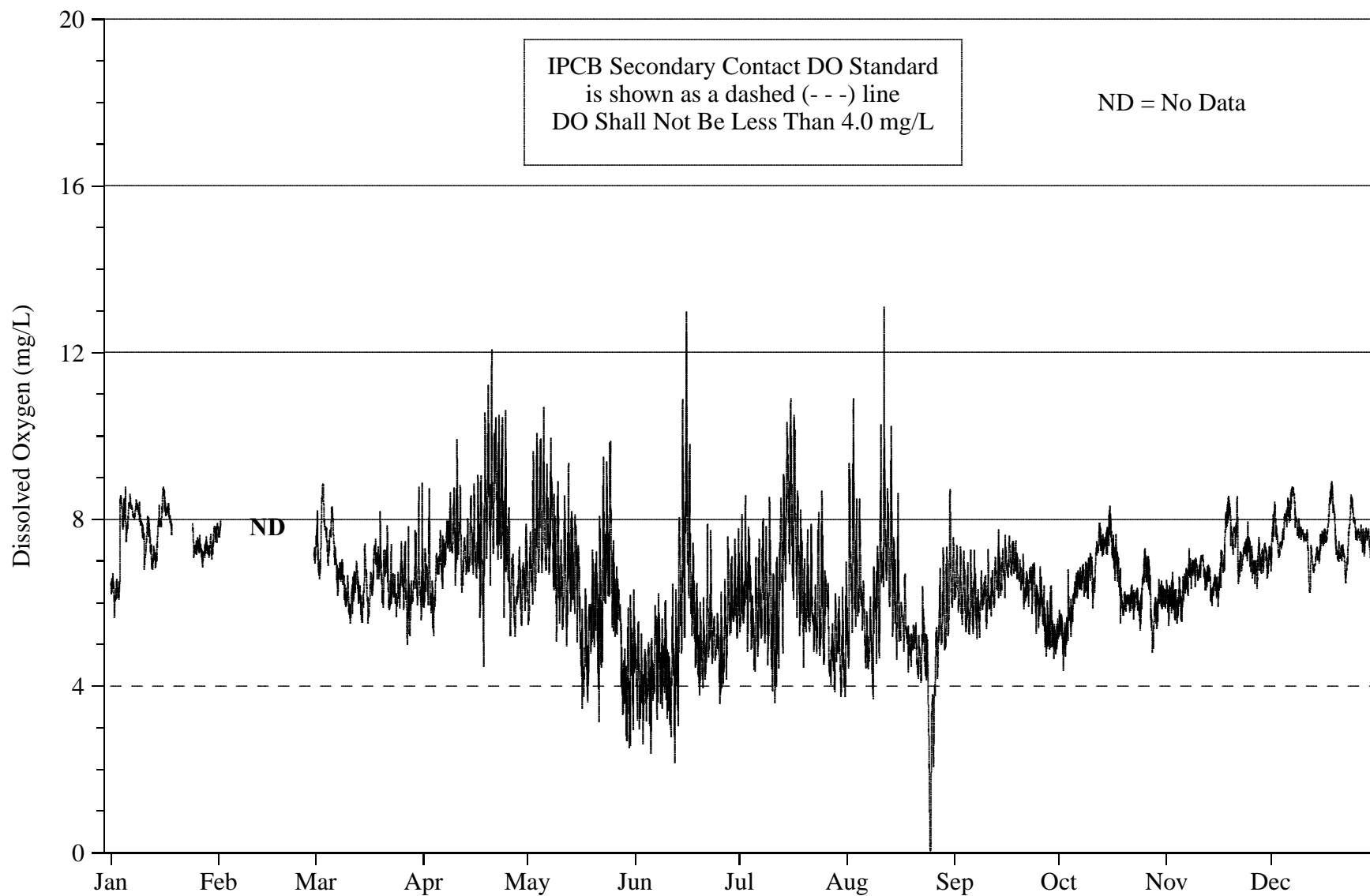
FIGURE 17: DISSOLVED OXYGEN CONCENTRATION MEASURED HOURLY AT HALSTED STREET ON THE LITTLE CALUMET RIVER FROM JANUARY 2007 THROUGH DECEMBER 2007
