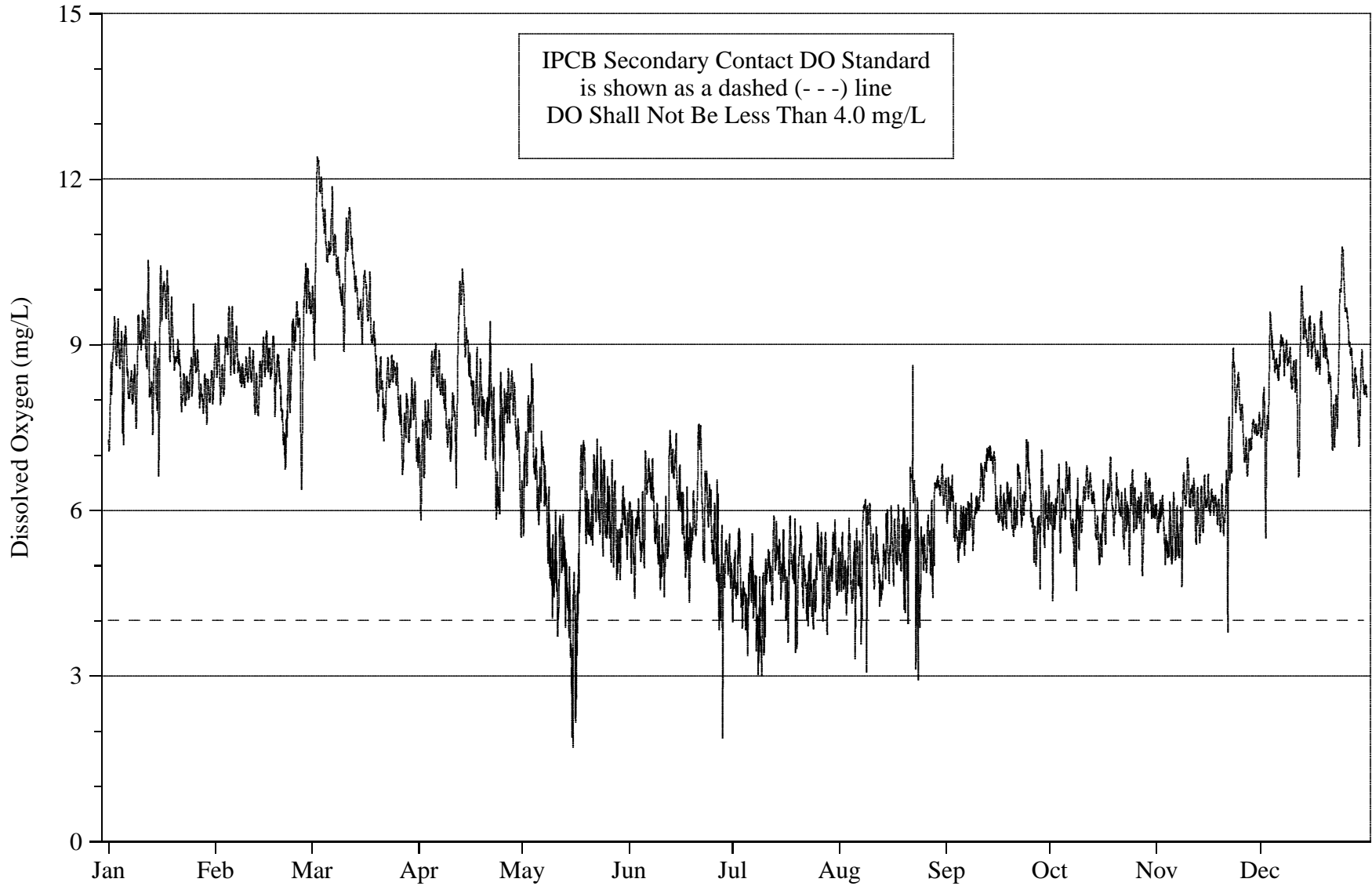
FIGURE 5: DISSOLVED OXYGEN CONCENTRATION MEASURED HOURLY AT FULLERTON AVENUE ON THE NORTH BRANCH CHICAGO RIVER FROM JANUARY 2007 THROUGH DECEMBER 2007
