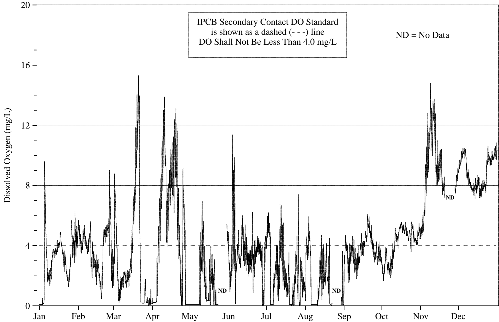
FIGURE 9: DISSOLVED OXYGEN CONCENTRATION MEASURED HOURLY AT 36TH STREET ON BUBBLY CREEK FROM JANUARY 2007 THROUGH DECEMBER 2007
