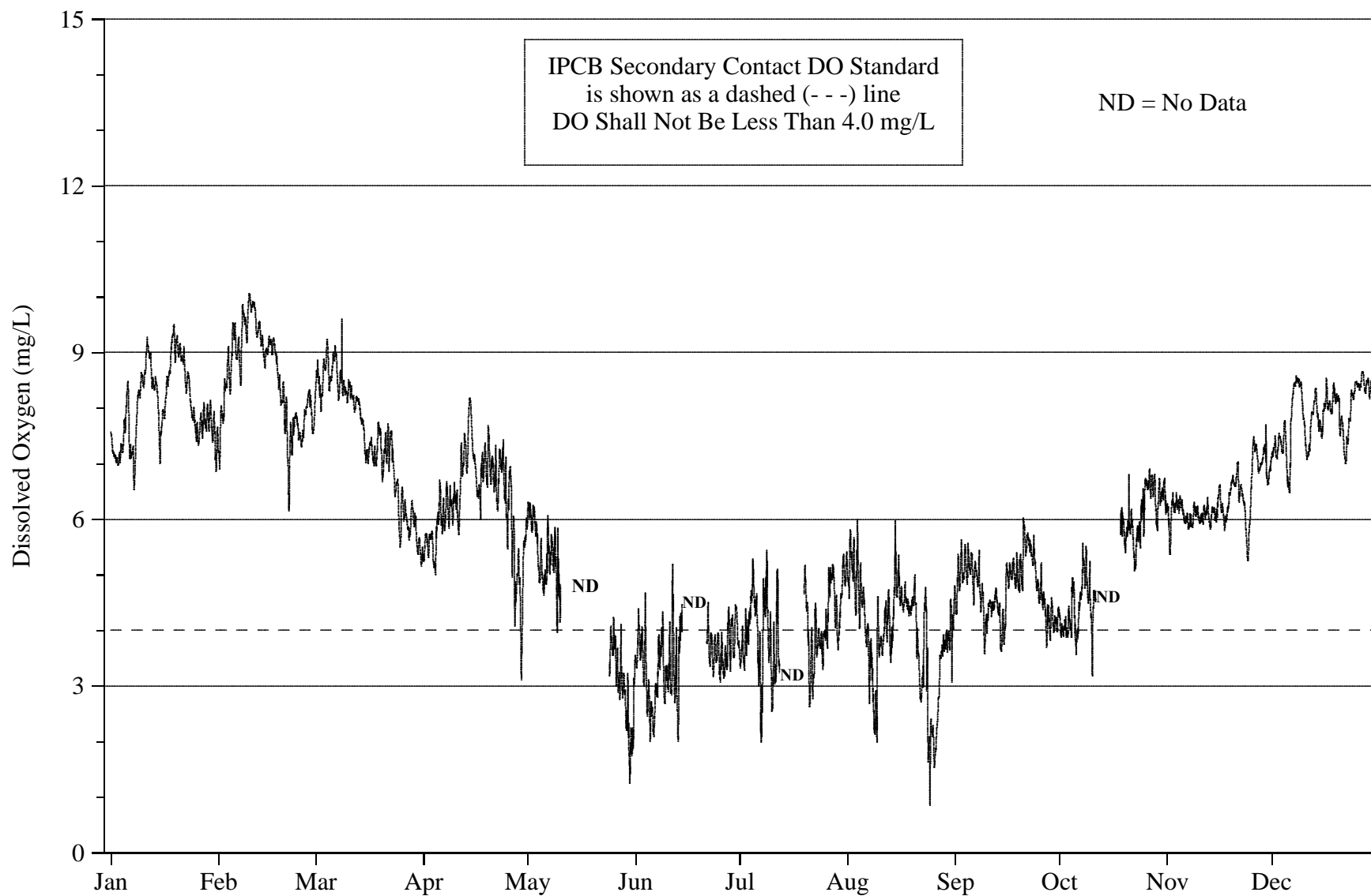
FIGURE 14: DISSOLVED OXYGEN CONCENTRATION MEASURED HOURLY AT LOCKPORT POWERHOUSE ON THE CHICAGO SANITARY AND SHIP CANAL FROM JANUARY 2007 THROUGH DECEMBER 2007
