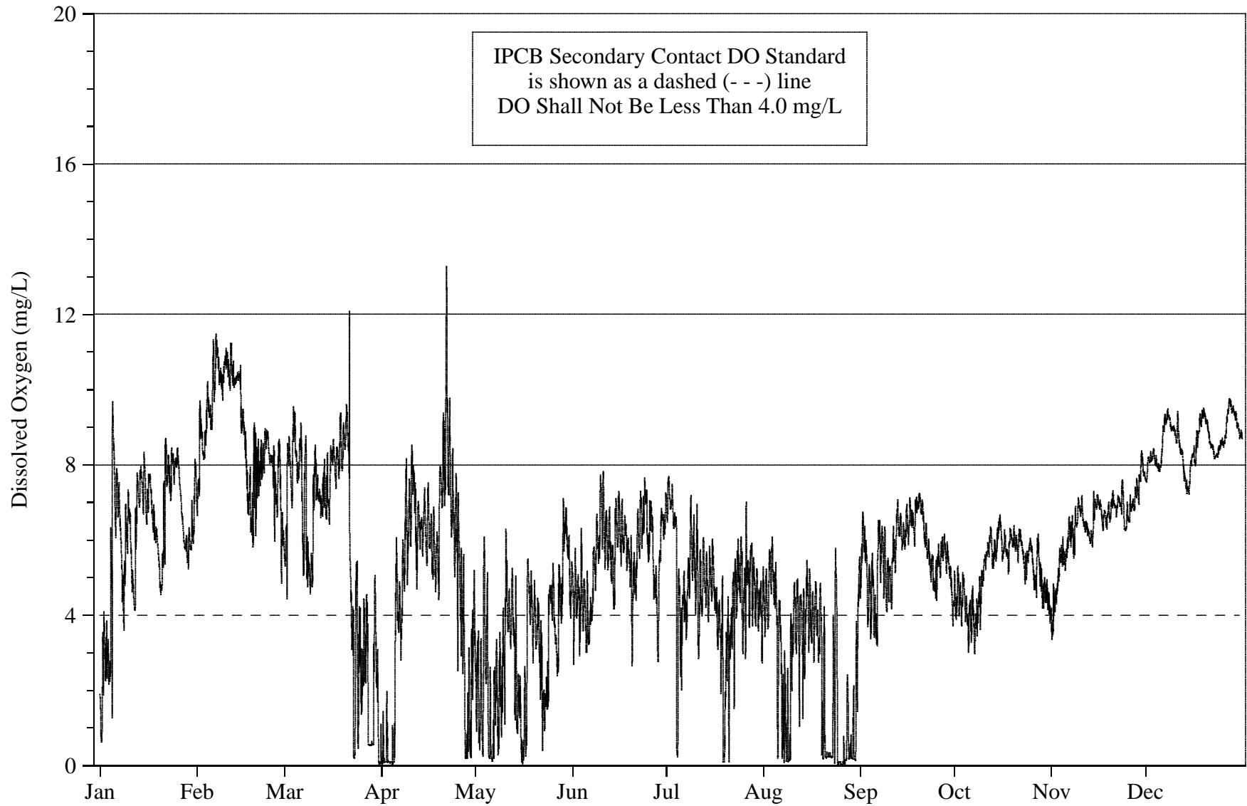
FIGURE 10: DISSOLVED OXYGEN CONCENTRATION MEASURED HOURLY AT INTERSTATE HIGHWAY 55 ON BUBBLY CREEK FROM JANUARY 2007 THROUGH DECEMBER 2007
