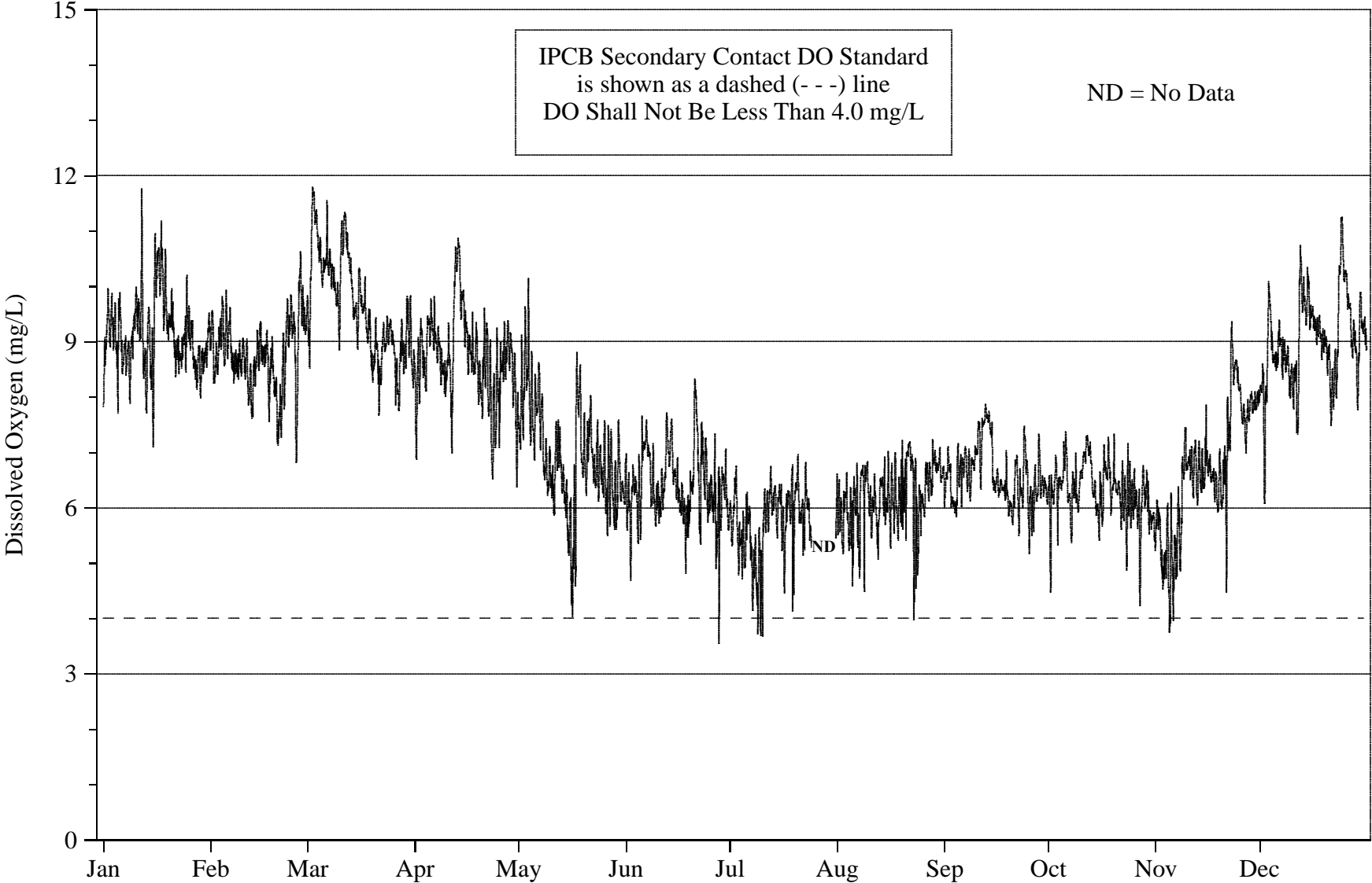
FIGURE 4: DISSOLVED OXYGEN CONCENTRATION MEASURED HOURLY AT ADDISON STREET ON THE NORTH BRANCH CHICAGO RIVER FROM JANUARY 2007 THROUGH DECEMBER 2007
