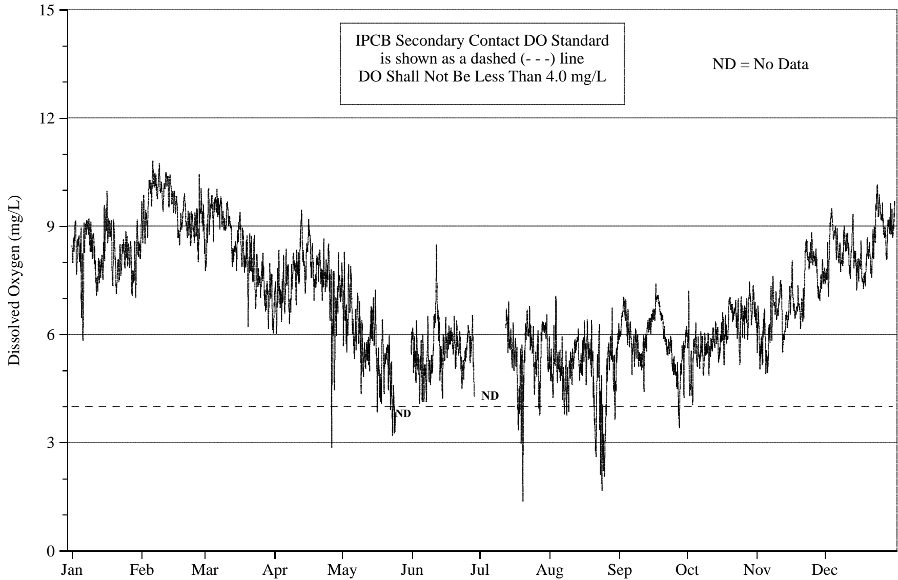
FIGURE 12: DISSOLVED OXYGEN CONCENTRATION MEASURED HOURLY AT B&O CENTRAL RAILROAD ON THE CHICAGO SANITARY AND SHIP CANAL FROM JANUARY 2007 THROUGH DECEMBER 2007
