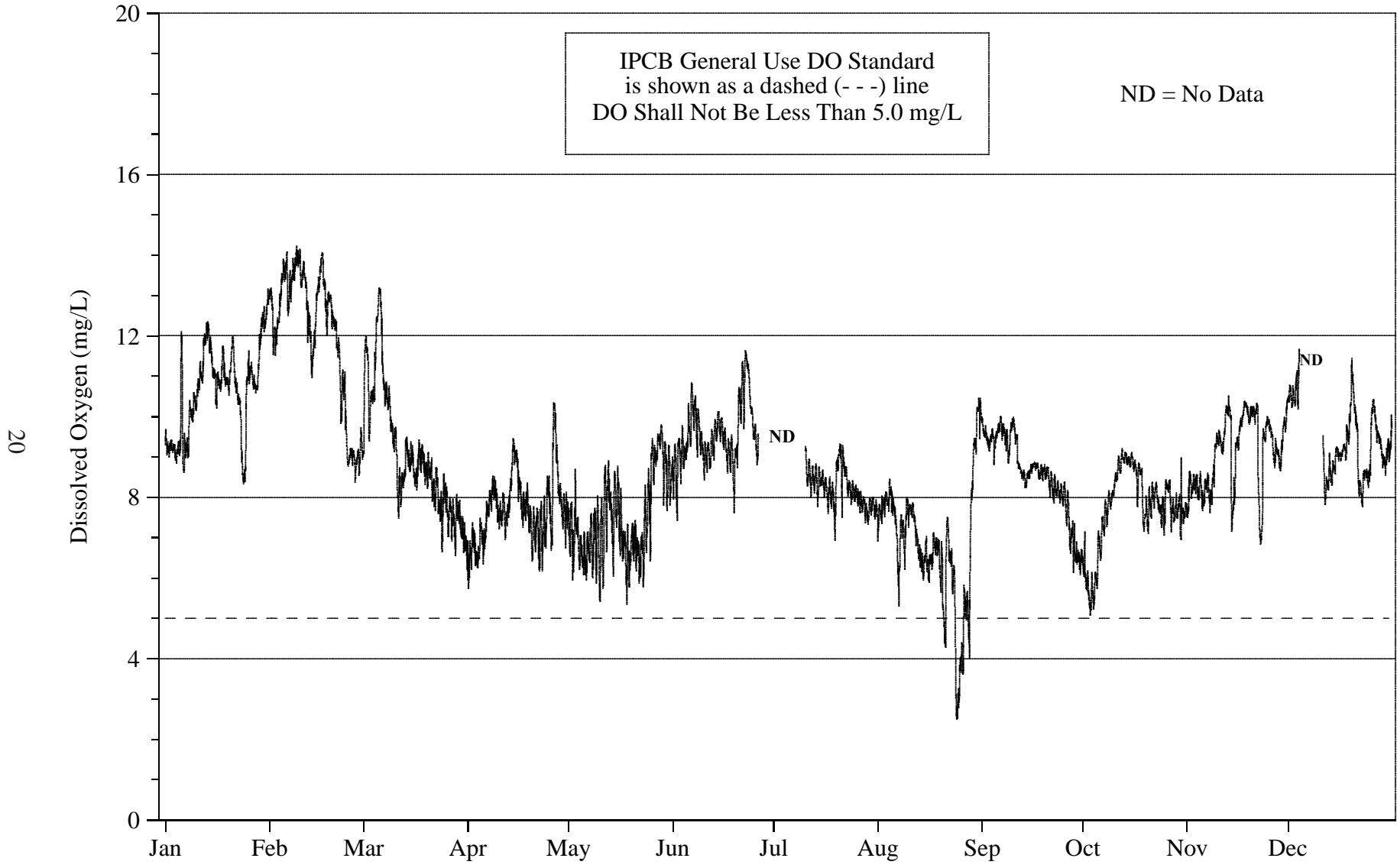
FIGURE 7: DISSOLVED OXYGEN CONCENTRATION MEASURED HOURLY AT CLARK STREET ON THE CHICAGO RIVER FROM JANUARY 2007 THROUGH DECEMBER 2007
