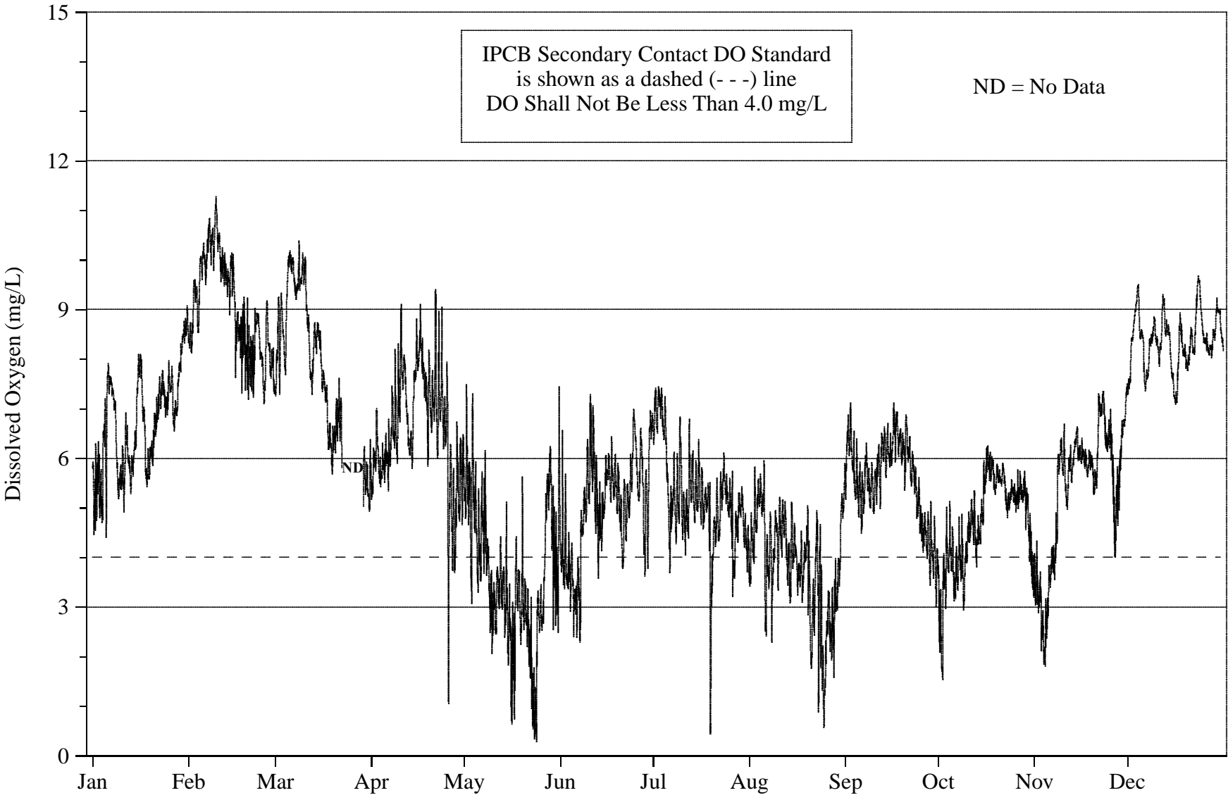
FIGURE 11: DISSOLVED OXYGEN CONCENTRATION MEASURED HOURLY AT CICERO AVENUE ON THE CHICAGO SANITARY AND SHIP CANAL FROM JANUARY 2007 THROUGH DECEMBER 2007
