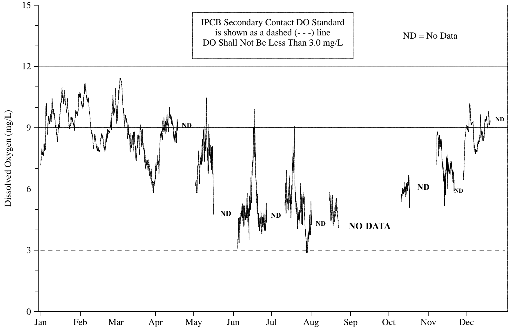
FIGURE 19: DISSOLVED OXYGEN CONCENTRATION MEASURED HOURLY AT 104TH AVENUE ON THE CALUMET-SAG CHANNEL FROM JANUARY 2007 THROUGH DECEMBER 2007
