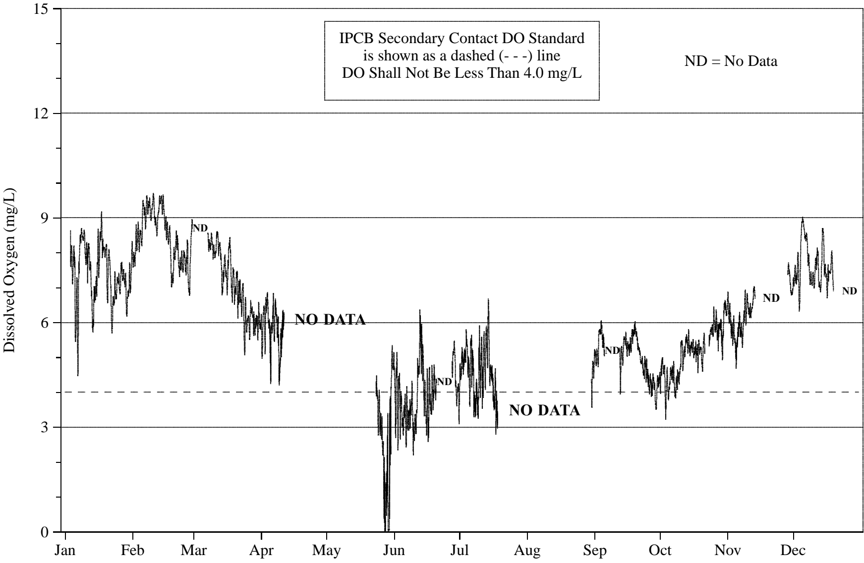
FIGURE 13: DISSOLVED OXYGEN CONCENTRATION MEASURED HOURLY AT ROUTE 83 ON THE CHICAGO SANITARY AND SHIP CANAL FROM JANUARY 2007 THROUGH DECEMBER 2007
