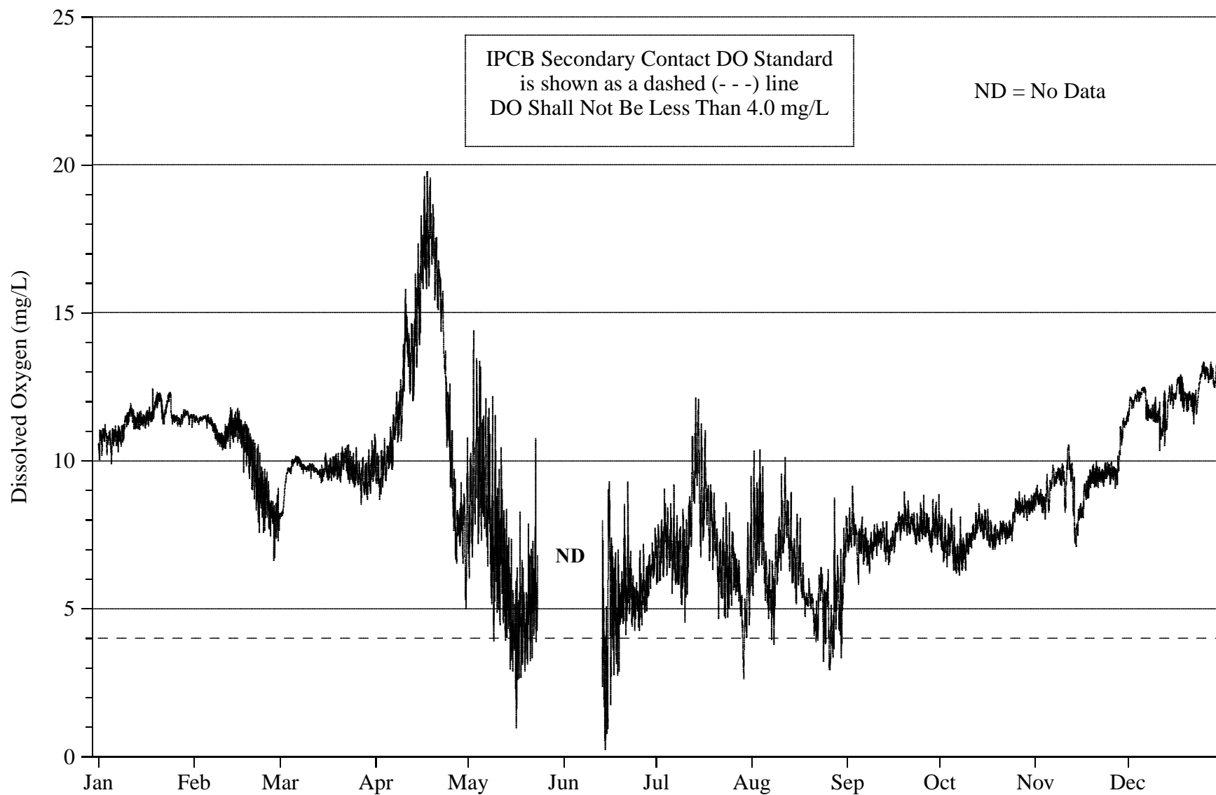
FIGURE 16: DISSOLVED OXYGEN CONCENTRATION MEASURED HOURLY AT C&W INDIANA RAILROAD ON THE LITTLE CALUMET RIVER FROM JANUARY 2007 THROUGH DECEMBER 2007
