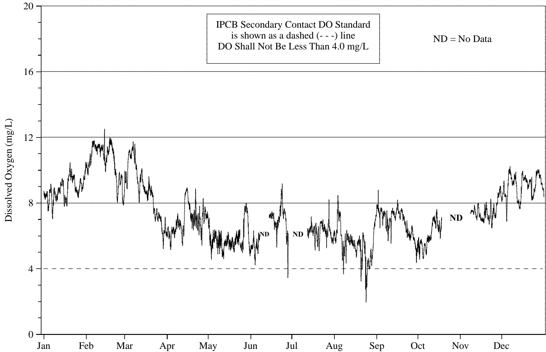
FIGURE 8: DISSOLVED OXYGEN CONCENTRATION MEASURED HOURLY AT LOOMIS STREET ON THE SOUTH BRANCH CHICAGO RIVER FROM JANUARY 2007 THROUGH DECEMBER 2007
