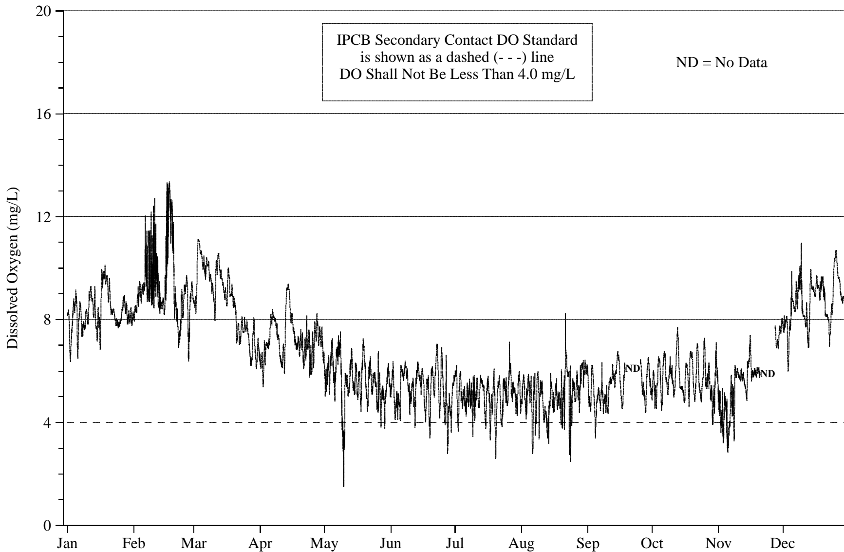
FIGURE 6: DISSOLVED OXYGEN CONCENTRATION MEASURED HOURLY AT KINZIE STREET ON THE NORTH BRANCH CHICAGO RIVER FROM JANUARY 2007 THROUGH DECEMBER 2007
